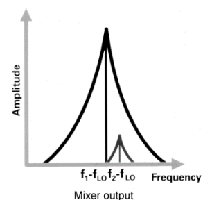
Figure 10. Phase noise masks the lower amplitude signal
