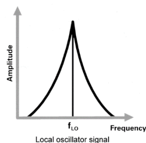
Figure 9. Local oscillator with phase noise
