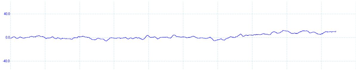
Figure 2. Phase stability between two 16 GHz RF signals locked to 10 MHz external reference
