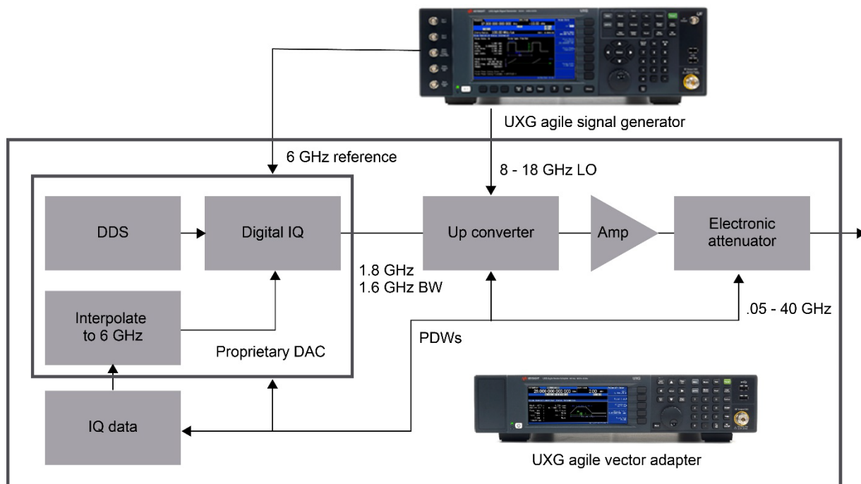
Figure 16. High-level block diagram of the UXG agile vector adapter
