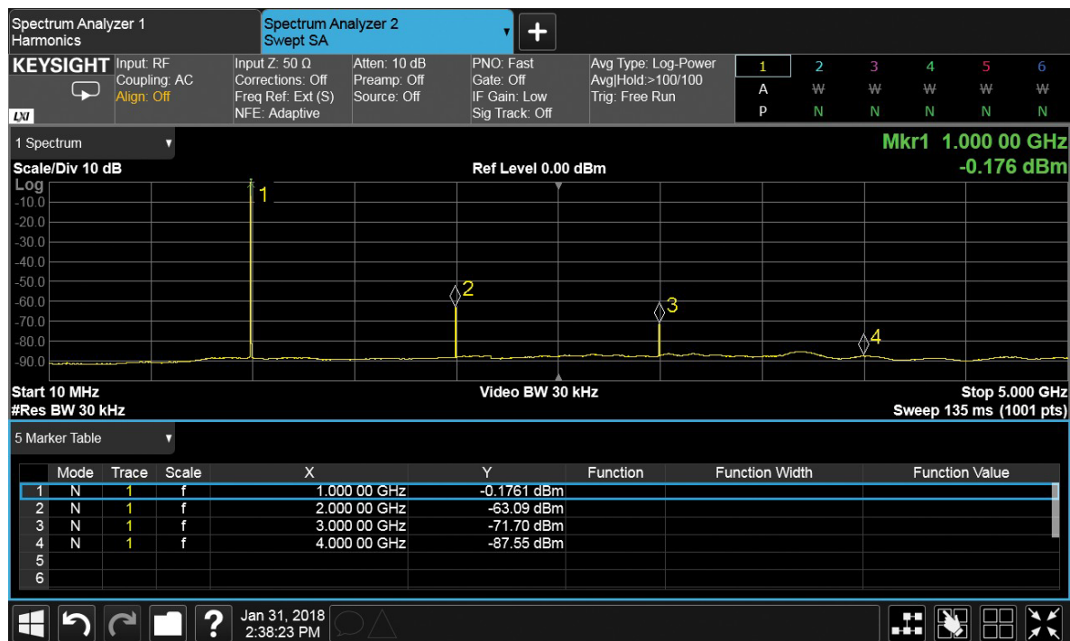
Figure 6. Spectrum analysis with frequency and amplitude readouts
