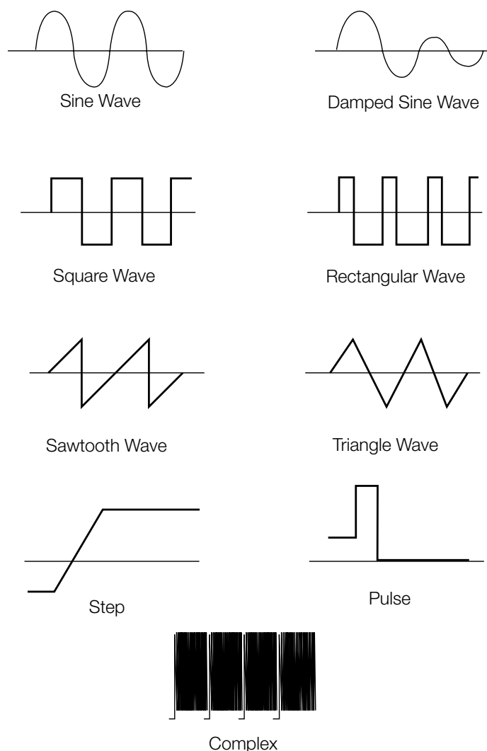
Figure 4. Common waveforms.
